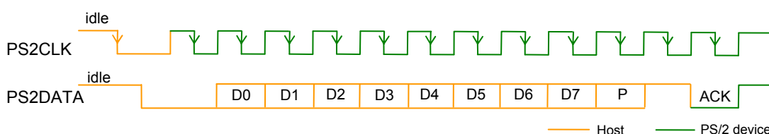
Figure 4. Transmission of data from Controller to PS/2 device
